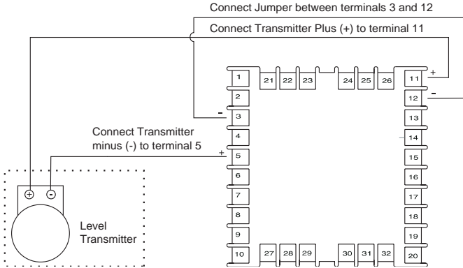
Figure 3 - Transmitter Wiring
