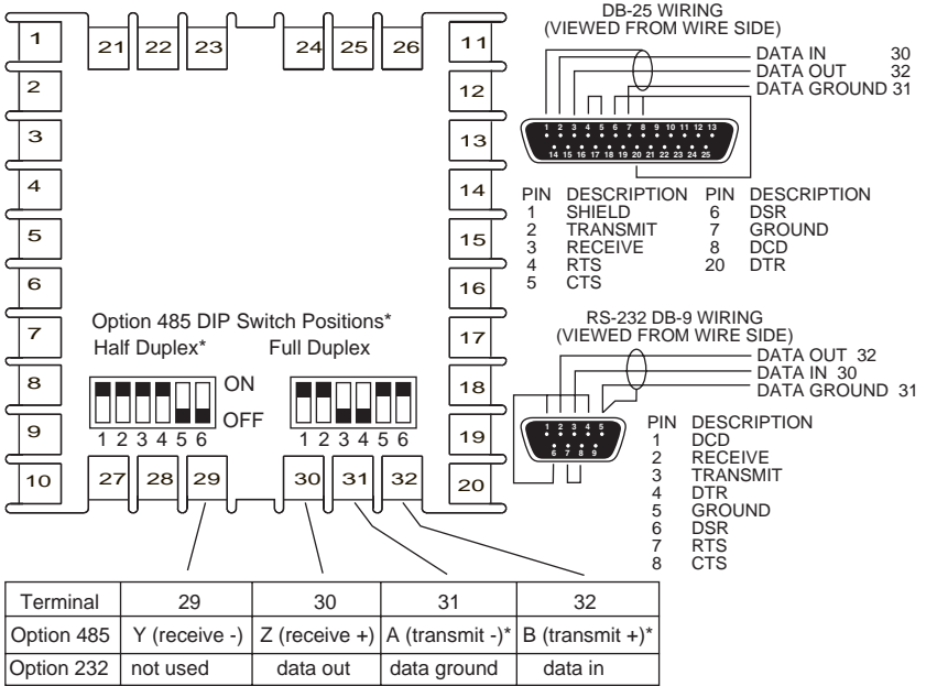
Figure 4 – Wiring for Options
