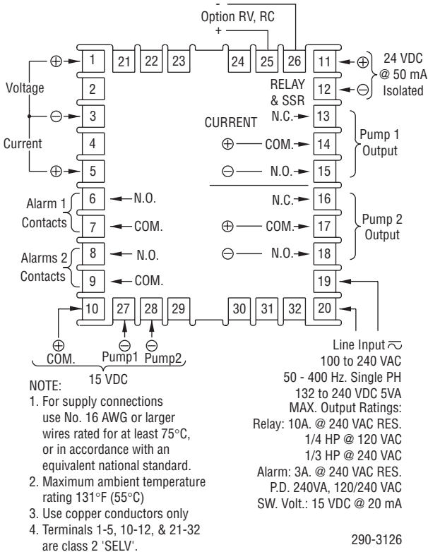
Figure 2 - Wiring
