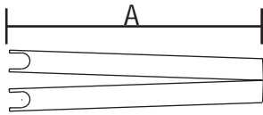
Web Type Surface Thermocouple Replacement Element
